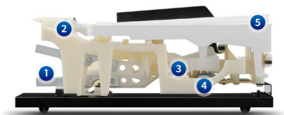
Mecanismo Responsive Hammer Compact
